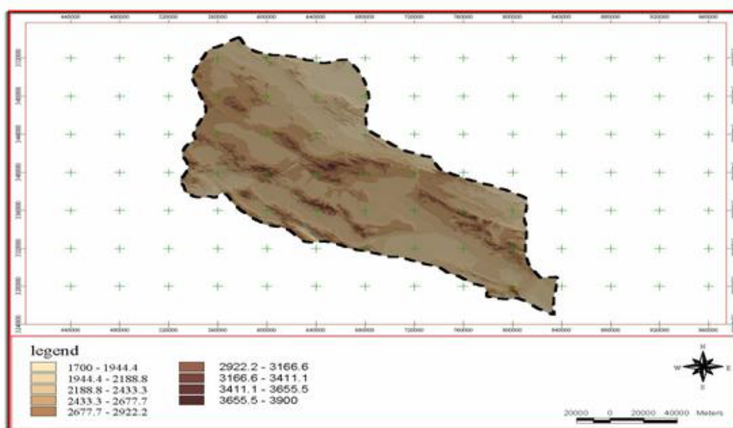
Fig. 3: Digital Elevation Model of the studied region
