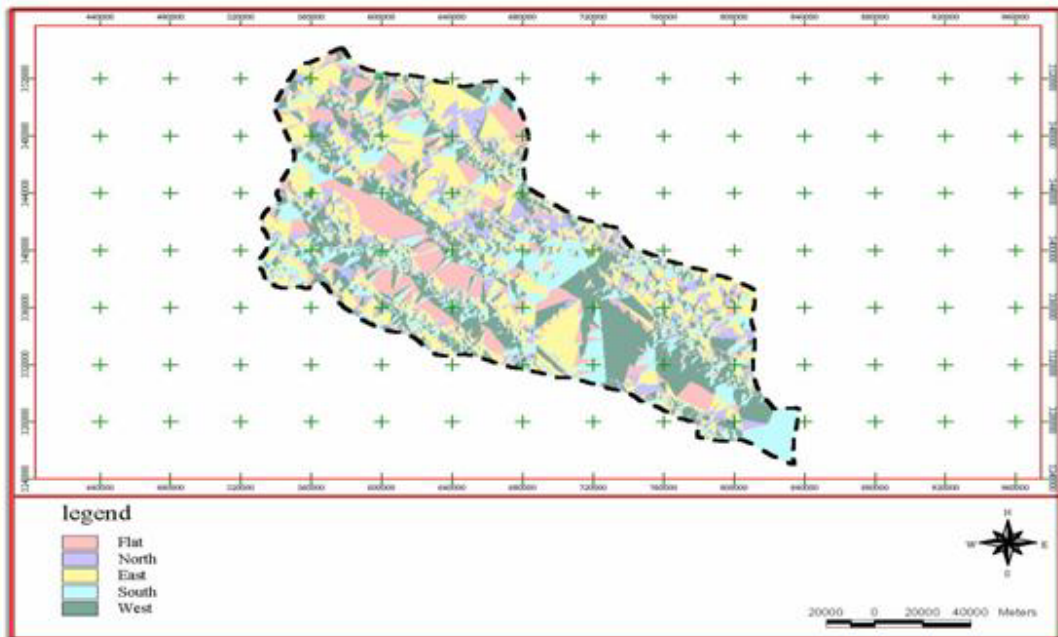
Fig. 5: Geographical aspect map in the studied region
