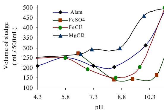
Fig. 2: Settled sludge volume for 400 mg/L of coagulants
