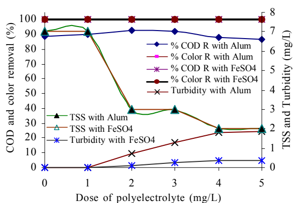
Fig. 5: Percentage removal of color and COD And TSS and turbidity for different doses of polyelectrolyte. (For 200 mg/L Alum or 200 mg/L of \text{FeSO}_4 )
