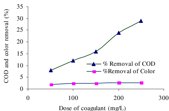
Fig. 6: Percentage removal of color and COD for different doses of lime (At pH= 10.3)
