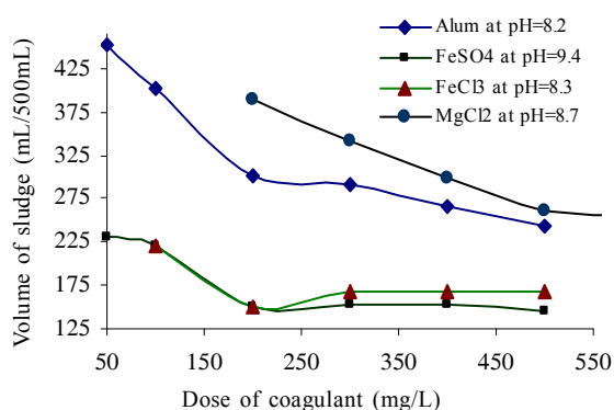
Fig. 4: Settled sludge volume for different coagulants at their optimum pH
