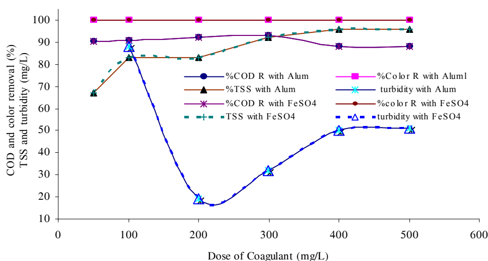
Fig. 3: Percentage removal of color, COD and TSS and turbidity for different doses of coagulant (At optimum pH=8.2 for Alum or at pH=9.4 for \text{FeSO}_4 )
